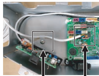
Remote Controller Connector (CN-REMO)
