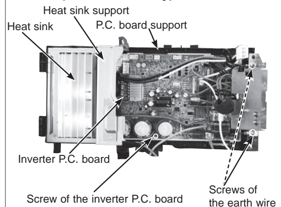
Photo 5 (Inverter assembly)
